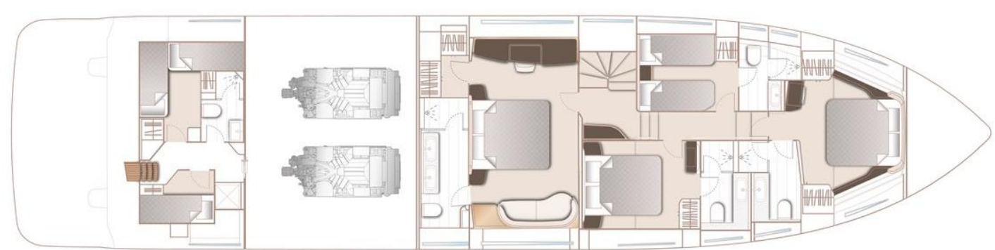
DECK 3
