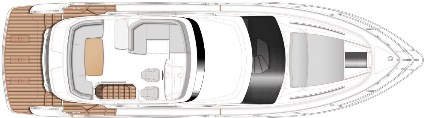
DECK 1
